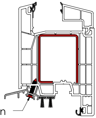
DRAINAGE PROFILE MONTAGE
