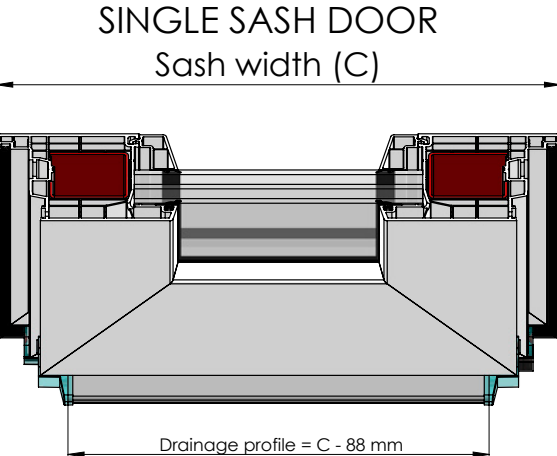
DRAINAGE PROFILE MONTAGE
