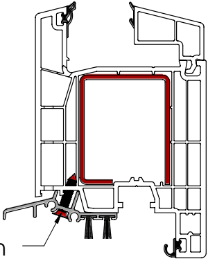
DRAINAGE PROFILE MONTAGE
